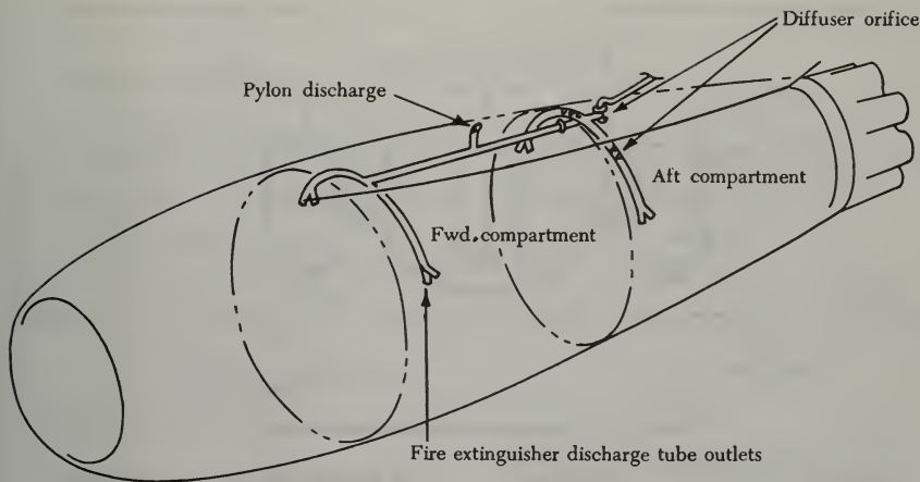
FIGURE 9-14. Fire extinguisher discharge tubes.
